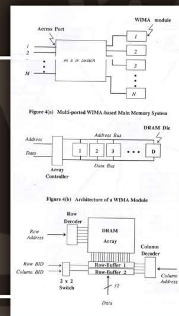
Wafer scale integrated memory architecture
