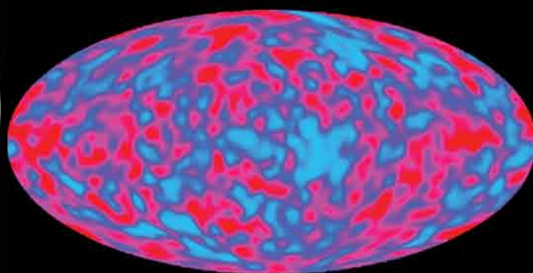
Cosmic microwave background map
