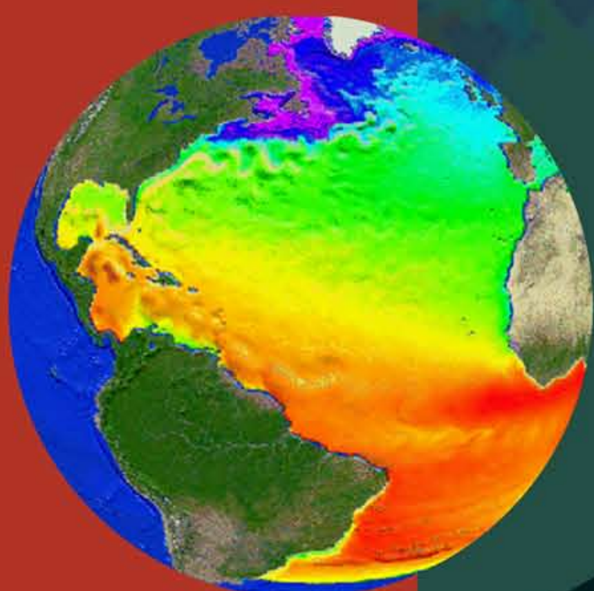
POP global climate model visualization
